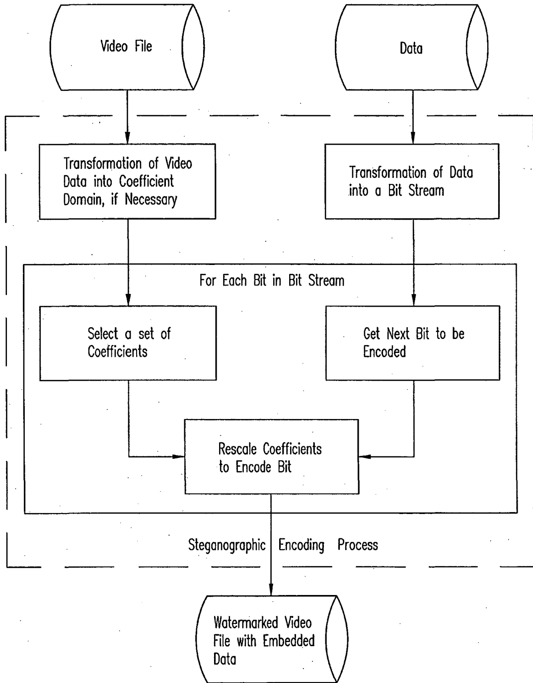
Encoding Data in a Video File
